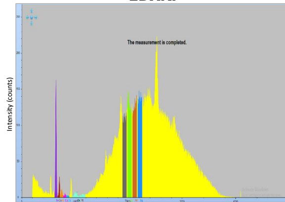
EDXRF
